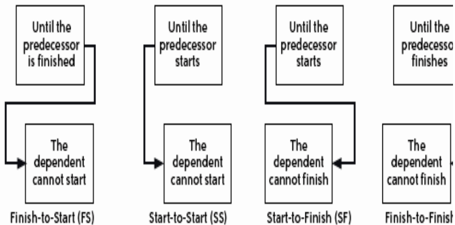
Figure 3.1: Task Dependency
