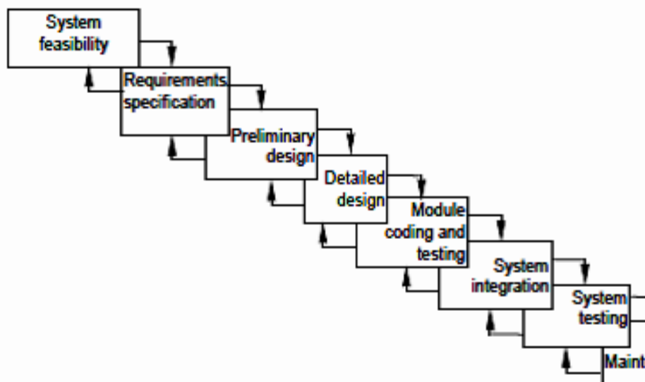
Figure 2.4 : Waterfall Model for Software Development
