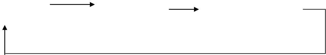
Figure 3.4 : Project Control
