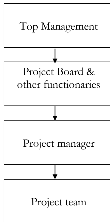
Figure 2.2 Organizational Structure
