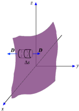
Fig 5: Infinite Sheet of Charge
