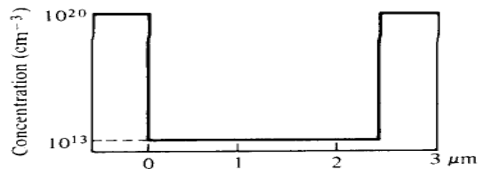
Doping profile
