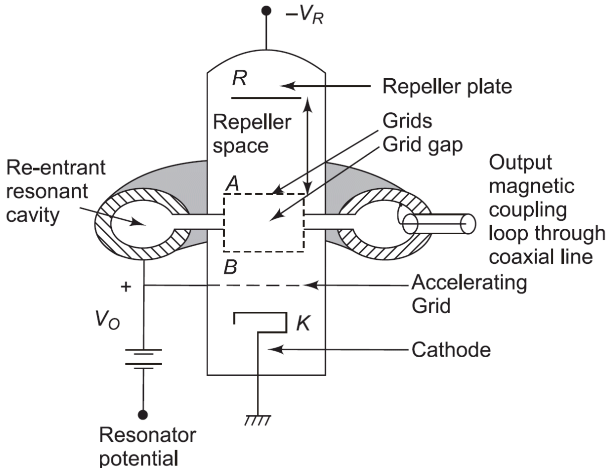
Fig. 9.3 Functional diagram of a reflex klystron
