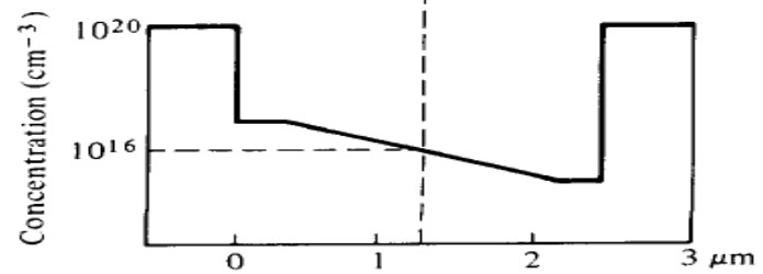
Doping profile
