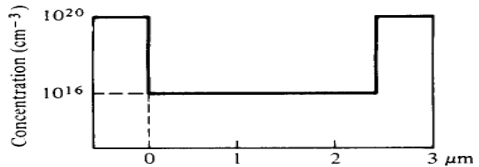
Doping profile
