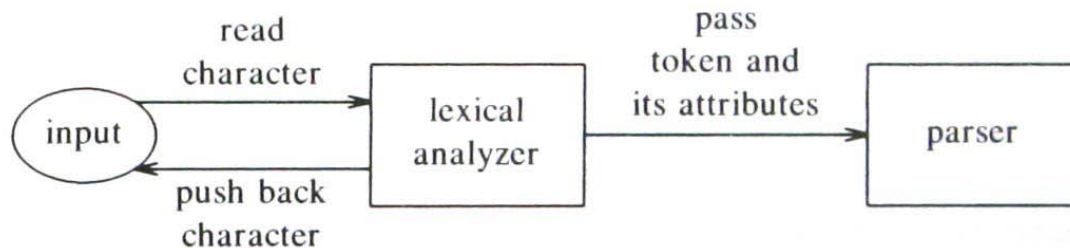
Fig 2.15. Inserting a lexical analyzer between the input and the parser
