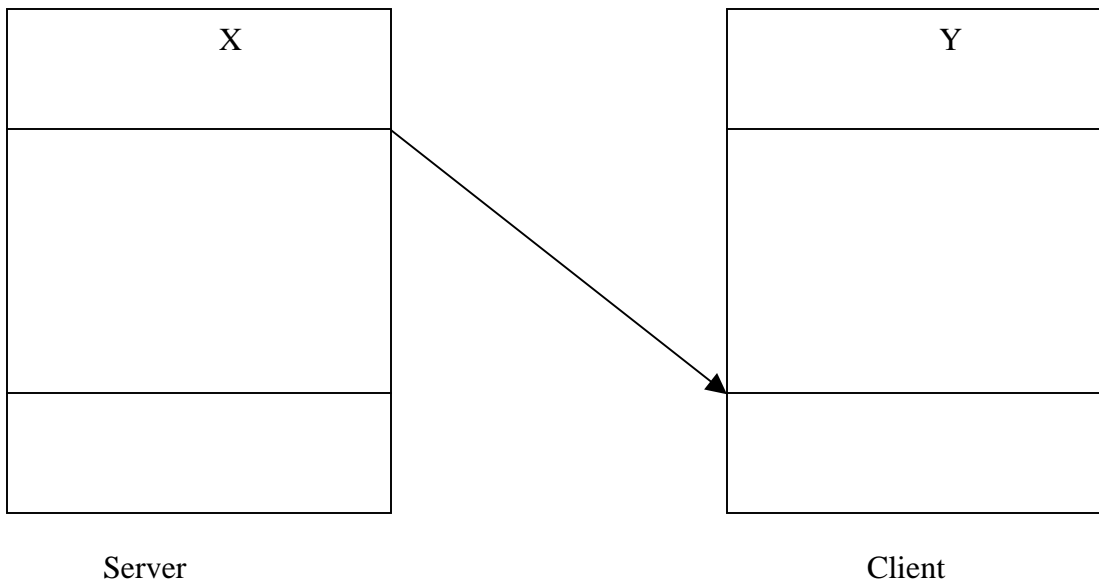
Fig. 7.13 Client-Server relationship
