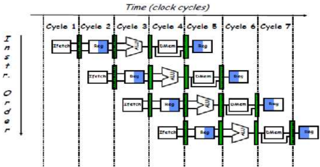
Figure 2.4 Pipeline activity
