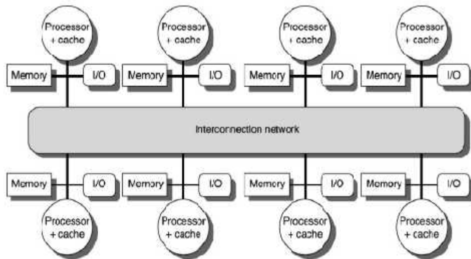
Distributed-memory multiprocessor
